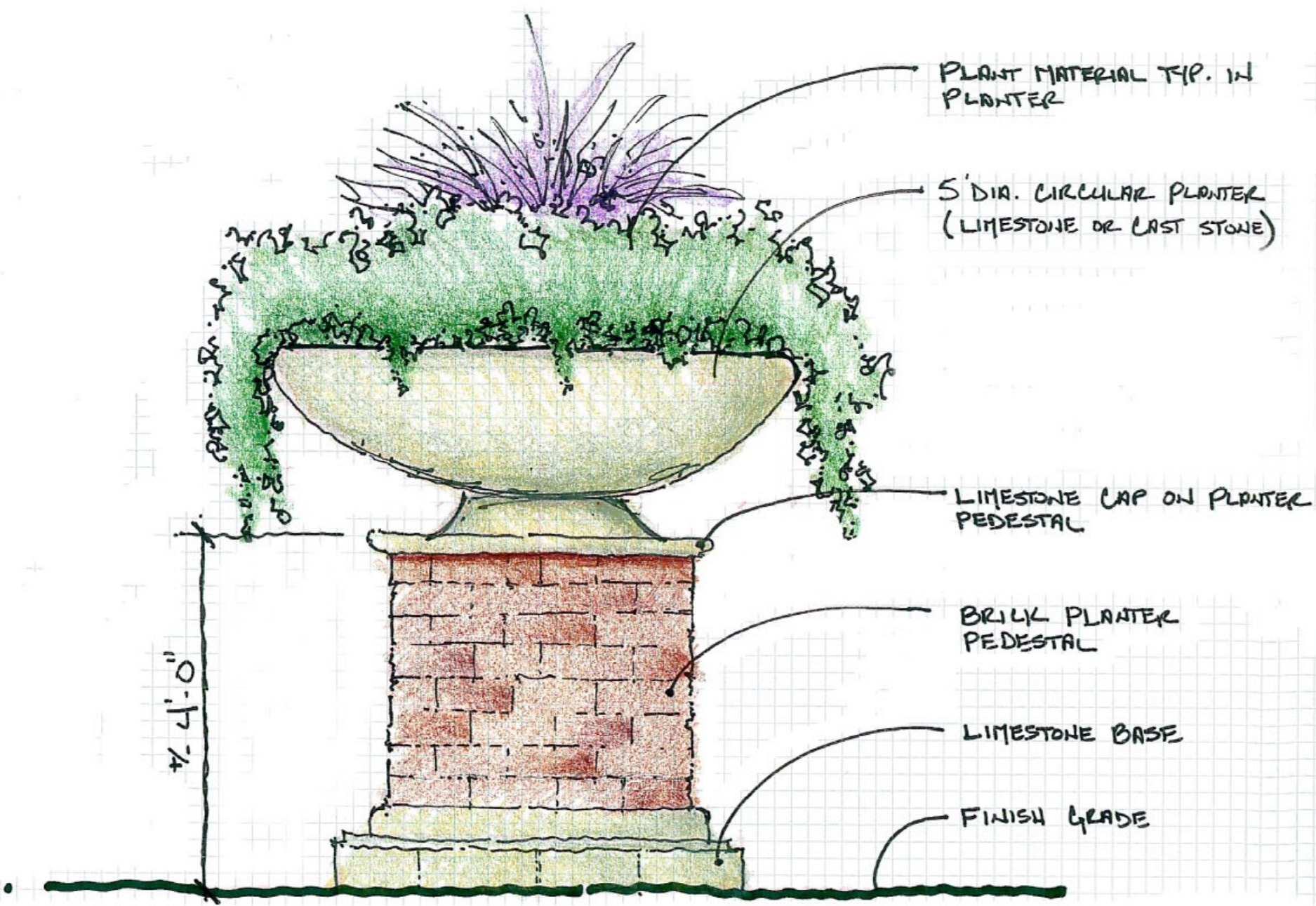
TYPICAL RAISED PLANTER
