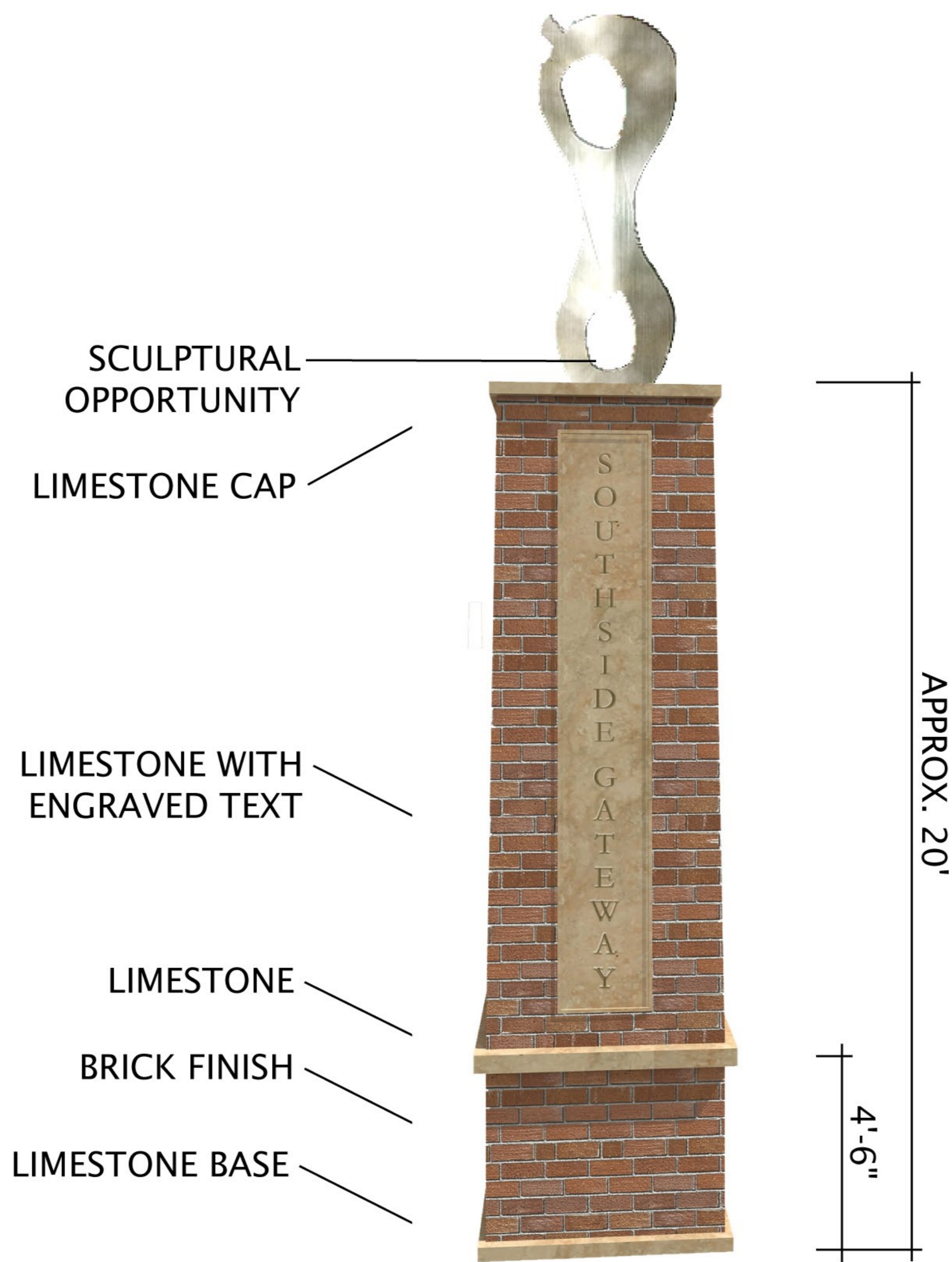
MONUMENT MARKER
