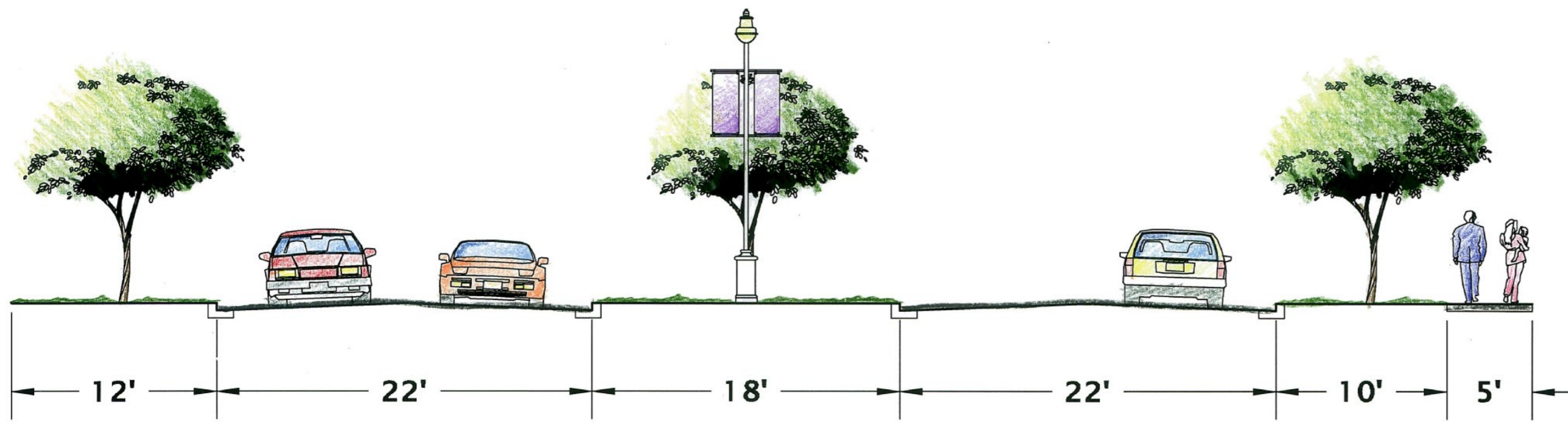
MADISON AVENUE WITH MEDIAN AND PEDESTRIAN WALKWAY
