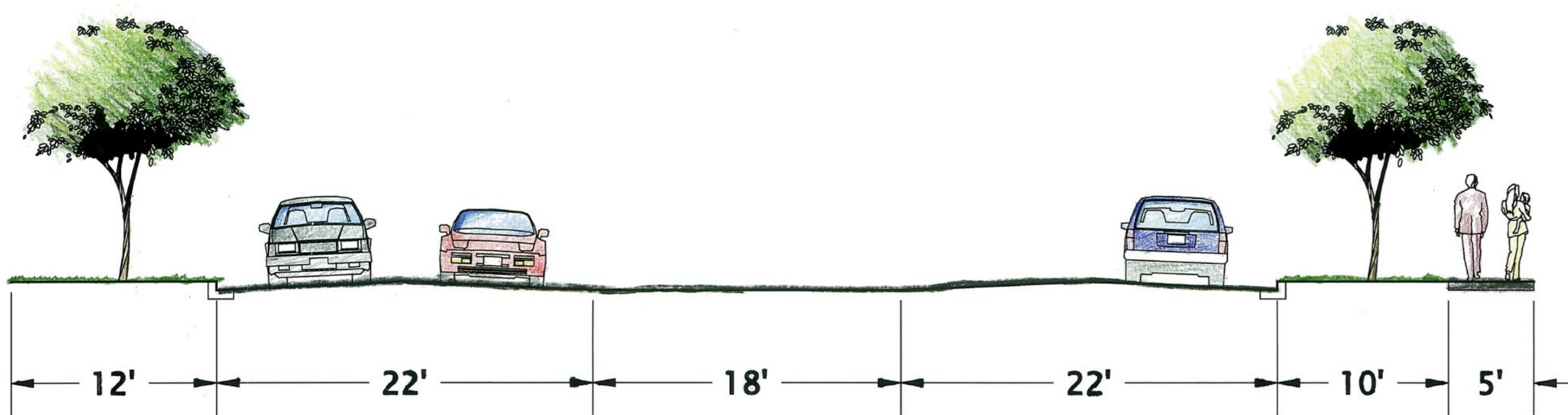
MADISON AVENUE WITH PEDESTRIAN WALKWAY
