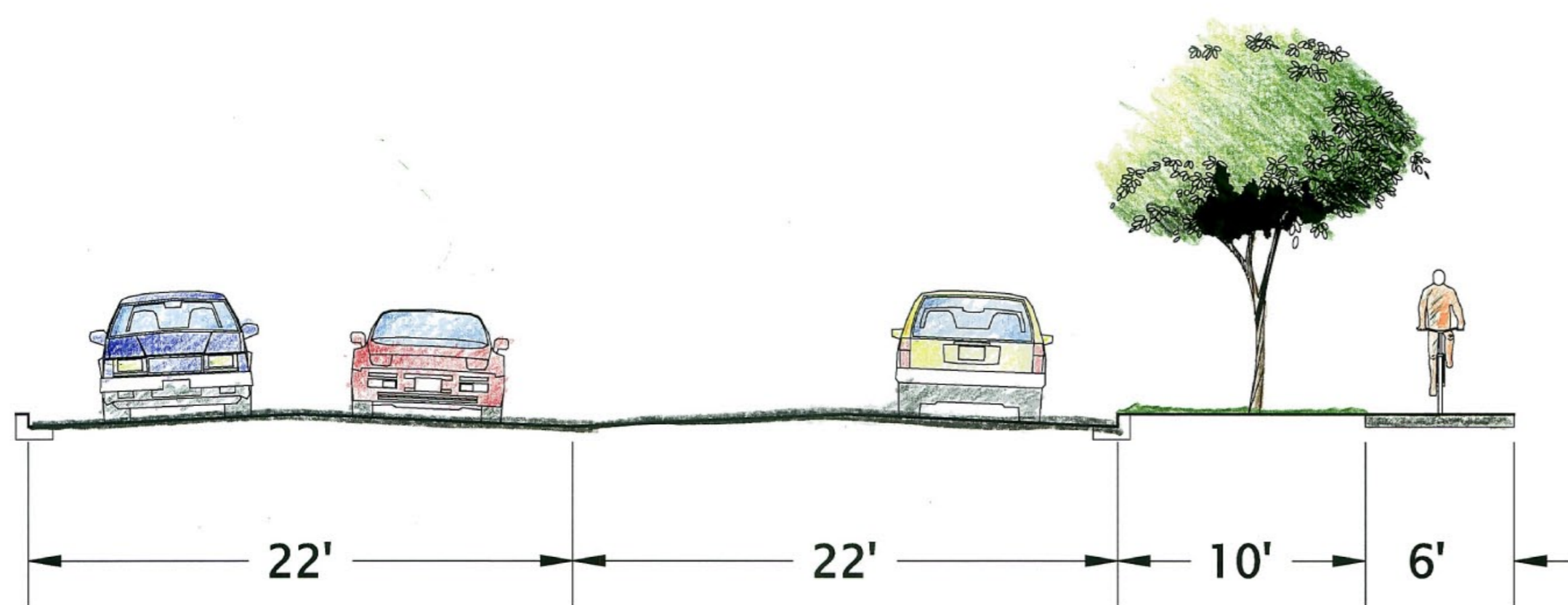
SHELBY STREET WITH BICYCLE LANE
